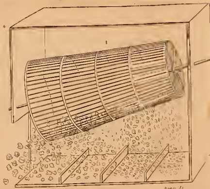
Cylinder for washing the Cusculliao .
